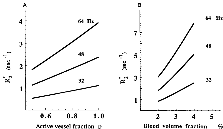
FIGURE 5 (A) The dependence of R_2^* on the active vessel fraction p in the capillary recruitment model ( b = 0.03 , vessel radius of 2.5\text{ }\mu\text{m} ). (B) The dependence of R_2^* on blood volume fraction for a constant population of blood vessels. The intercapillary distance was held constant at 31\text{ }\mu\text{m} , equivalent to that used for b = 0.02 with a cylinder radius of 2.5\text{ }\mu\text{m} . Increases in blood volume are produced by increases in vessel radius. This corresponds to the dilation model. The values of the shift frequency \nu are indicated in the figures.
